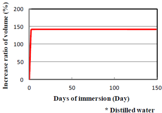
Figure 3: Long term swelling characteristics Leakmaster LV-Z
