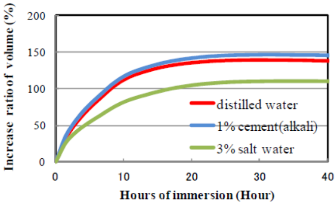
Figure 1: Swelling properties in various solutions of Leakmaster LV-Z
