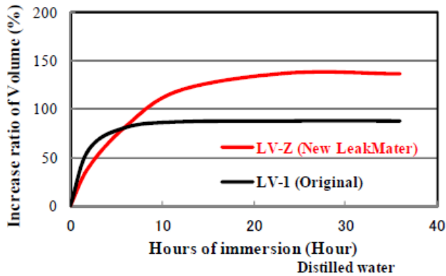
Figure 2: A difference of water swelling property
