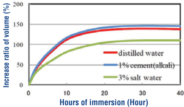
Swelling properties in various solutions of LEAKMASTER LV-Z
