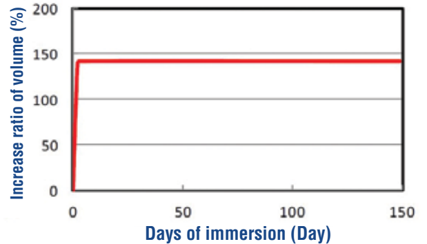
Long term swelling characteristics of LEAKMASTER LV-Z (distilled water)
